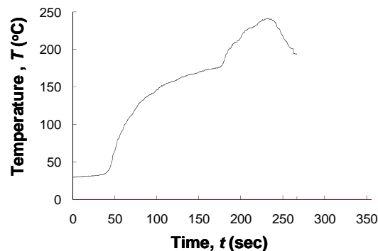
Figure 1. Temperature profile of a reflow process.
